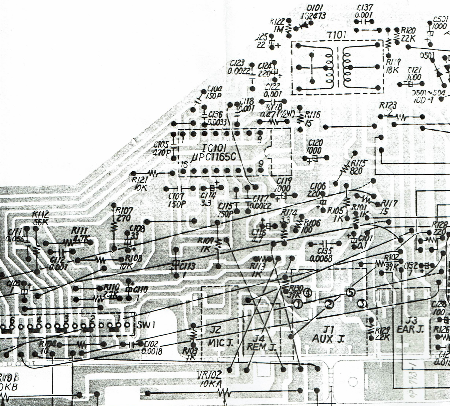
P.C.B. 2 OP-793 Bottom View
